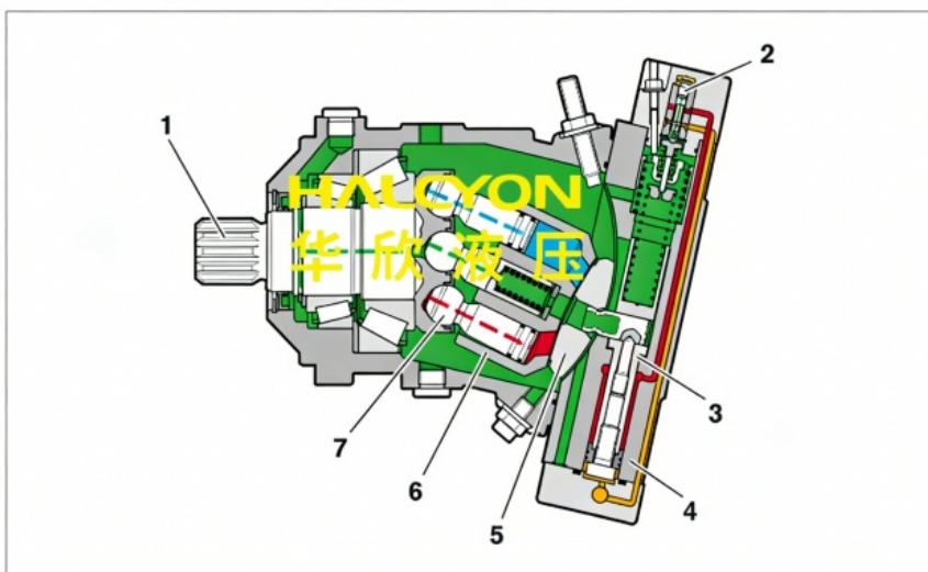
Fig. 2: Assembly of the A6VM
